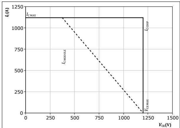
figure 49. IGBT
